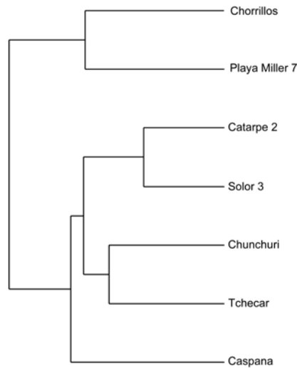
Figure 2: UPGMA tree based on the geometric morphometrics distance between the consensus configurations of the sites.
